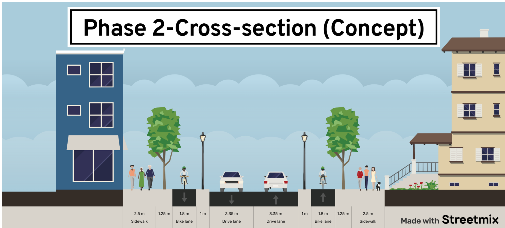
Figure 2- Sample picture of a cross-section with travel lanes and curb separated cycling lanes
