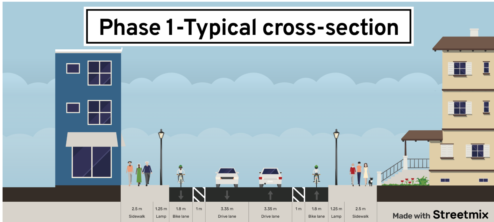
Figure 1– Cross-section of Benton Street showing travel lanes, painted buffer and cycling lanes
